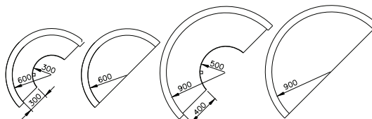
Radius Versions curve 180°
