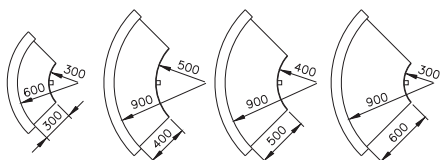
Radius Versions curve 90°
