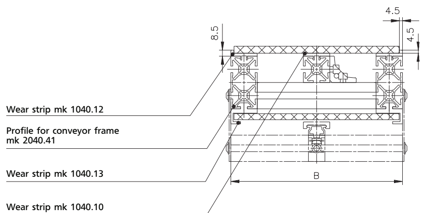
Conveyor frame cross-section
