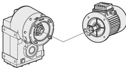
Flexible joint
