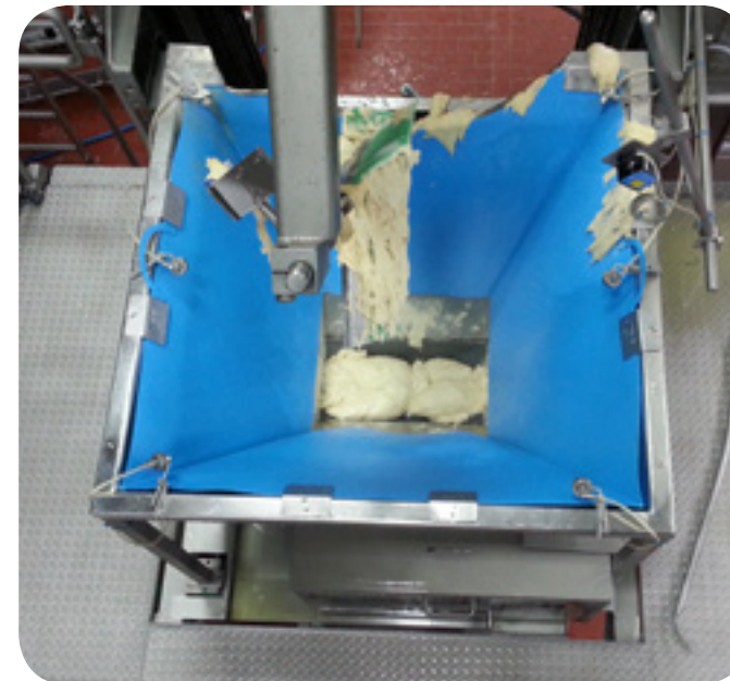
Hooper lining
