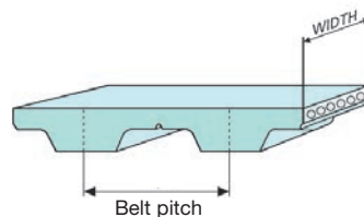
Reference dimensions
