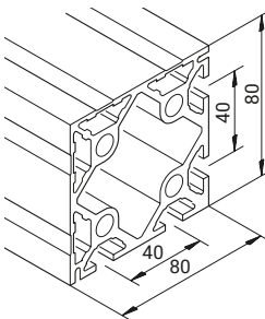
Profile mk 2040.13 (80x80)
