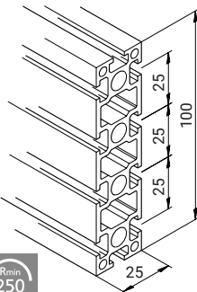
Profile mk 2025.03 (25x100)
