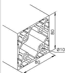
Profile mk 2040.109 (80x80)
