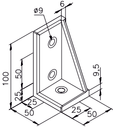
Angle bracket 1 31.00.0001
