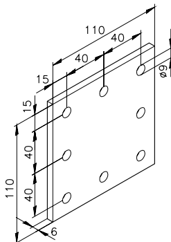
Connection plate 40/4 50.05.0062
