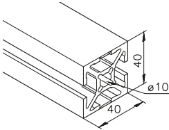
Profile mk 2040.94 (40x40)
