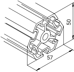
Profile mk 2025.20
