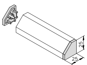
End cap for mk 2025.38 profile 25.50.8005
