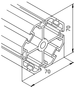
Profile mk 2025.21
