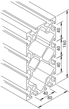
Profile mk 2040.08 (80x160)
