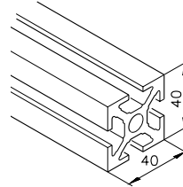
Profile mk 2040.01 (40x40)
