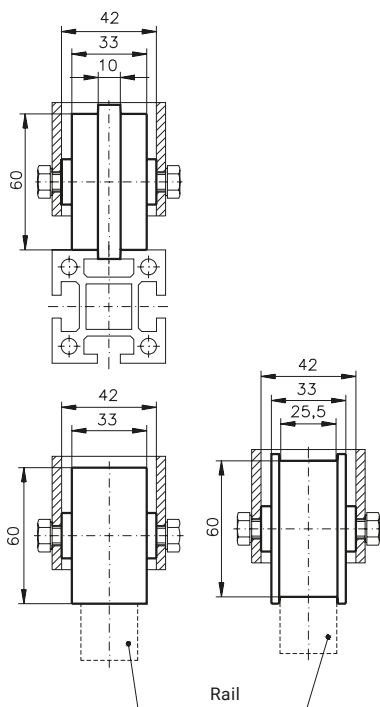
Fastening example
