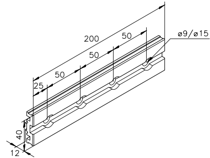
Connection plate 40/7 50.05.0065
