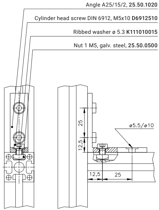
Fastening example set T25.50.1020
