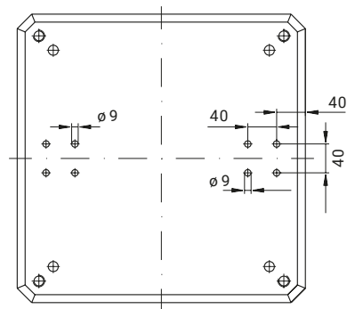
Sample drilling pattern
