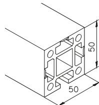
Profile mk 2017 (50x50)
