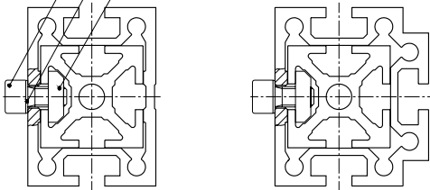
mk 2040.75 and mk 2040.01 profiles
