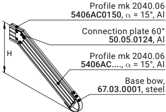
Side wall 40/30° B02.34.006
