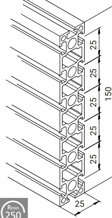
Profile mk 2025.04 (25x150)
