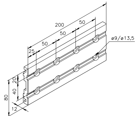
Connection plate 40/8 50.05.0066
