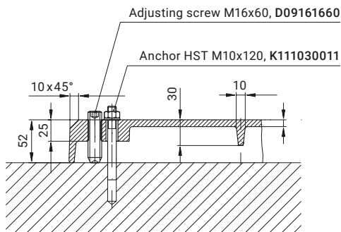
Fastening example
