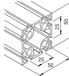
Profile mk 2025.05 (50x50)
