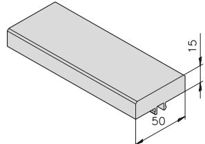
25|40|50|60 Wear strip mk 1071 22.71.2000
