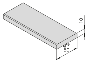
25|40|50|60 Wear strip mk 1070 22.70.2000
