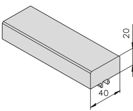
25|40|50|60 Wear strip mk 1040.04 21.04.2000
