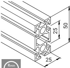
Profile mk 2025.02 (25x50)
