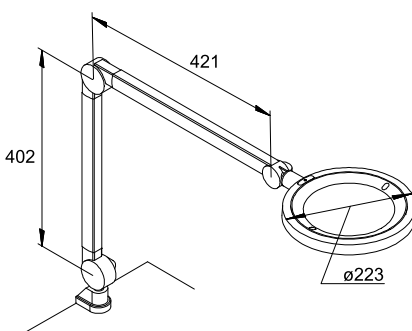
LED illuminated magnifying glass B02.23.807
