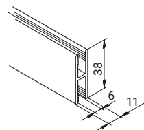
Profile mk 2215
