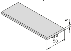
25|40|50|60 Wear strip mk 1001 22.01.2000
