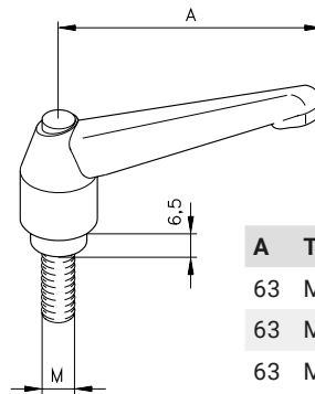
Clamping lever, die-cast zinc
