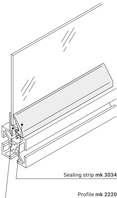
Fastening example
