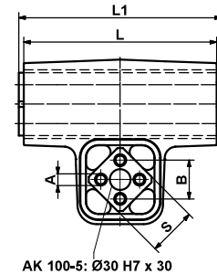
AK 100-5: Ø30 H7 x 30
