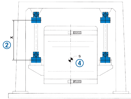
Hanging and freely oscillating gyratory sifter
